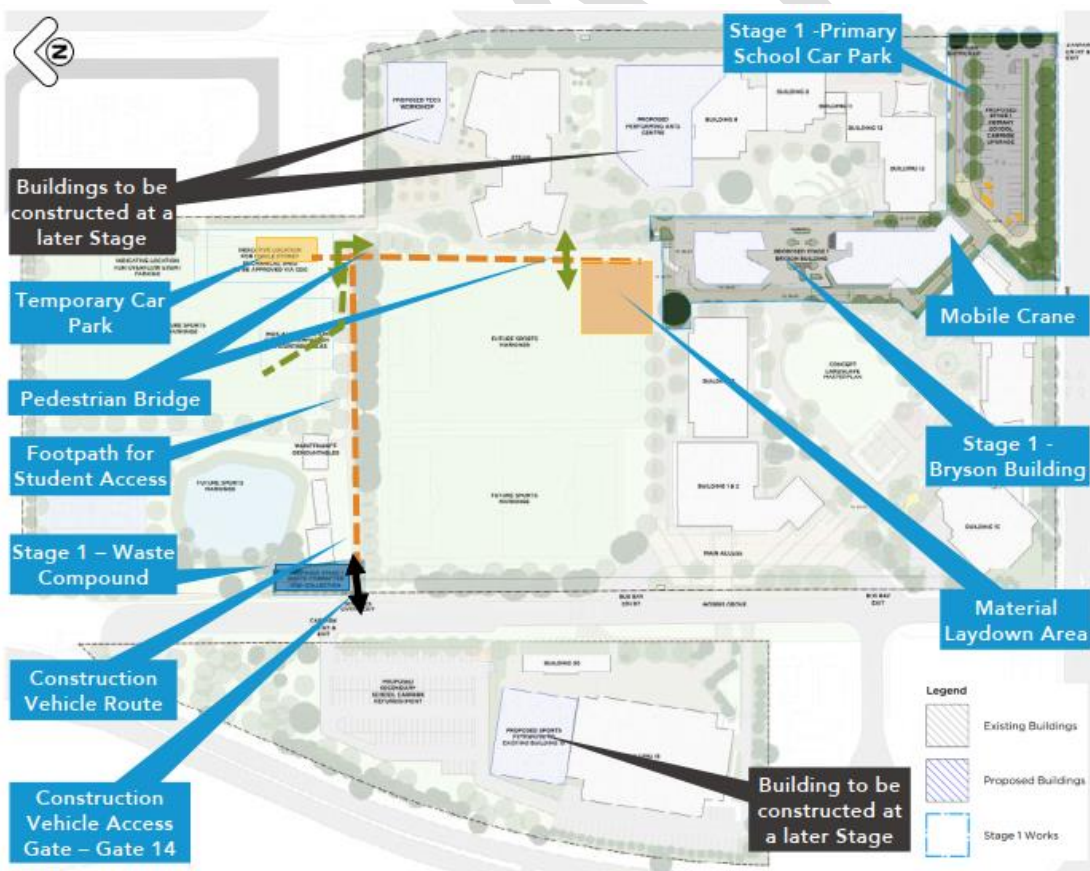
Figure 3.1 Construction activities Stage 1 (note carpark and waste compound not included in this scope or plan)
