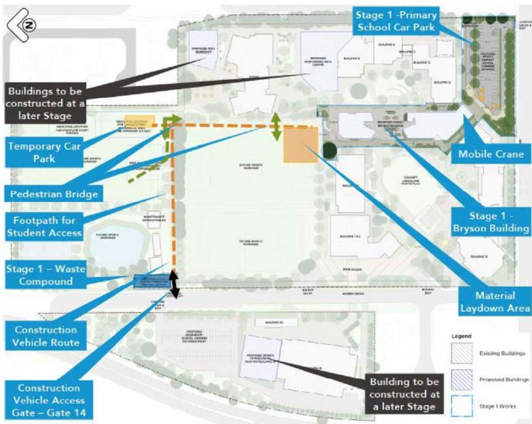
Source: William Clarke College Traffic Impact Assessment (PTC, June 2023)
